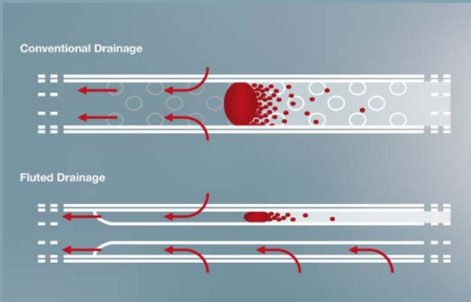
SecuroPlus fluted low-vacuum drainage
